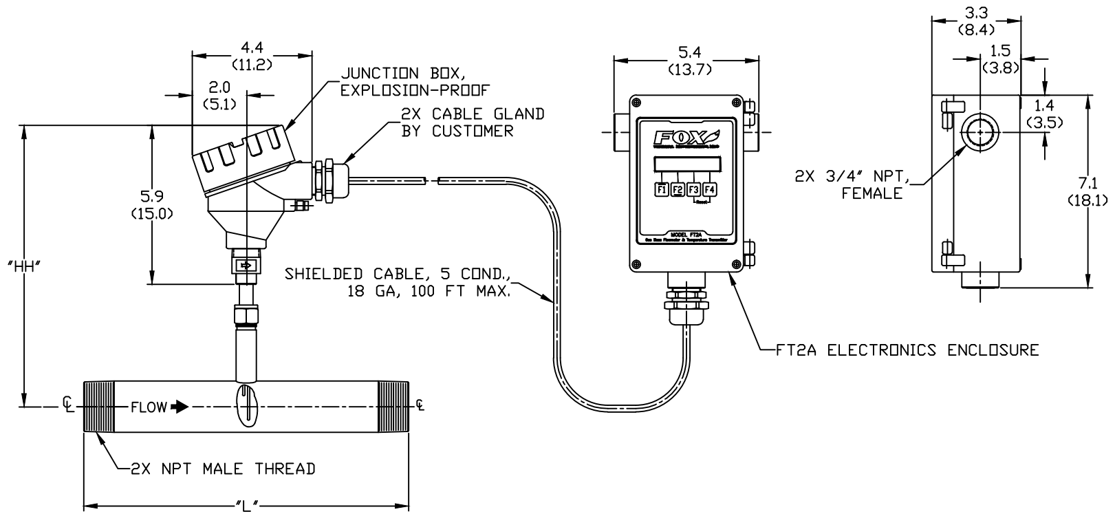
FT2A INLINE FLOWMETER, NPT END CONNECTIONS, REMOTE ELECTRONICS
