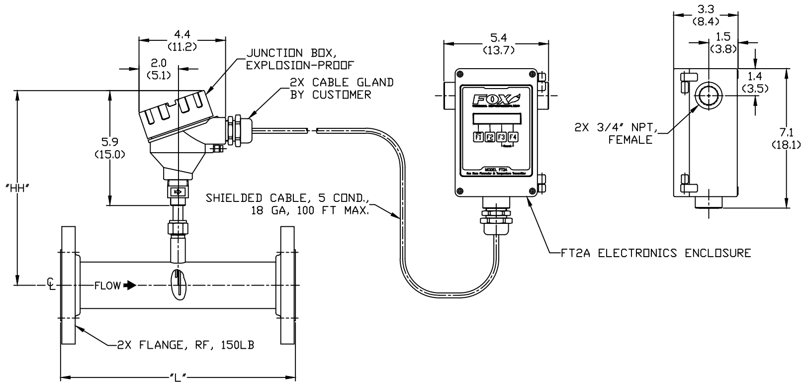
FT2A INLINE FLOWMETER, 150# FLANGE CONNECTIONS, REMOTE ELECTRONICS
